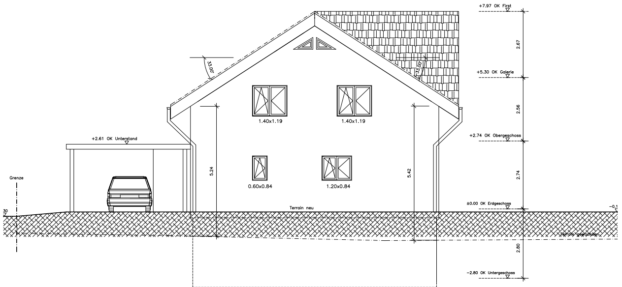
WEST FASSADE
